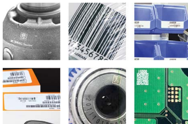
Figure 6. Code substrates affect reflectance differently and influence lighting angles.
